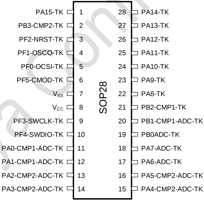
图 3-4 SOP28 Pinout2 PY32T020G2xS7 (Top view)
