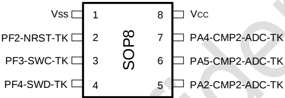
图 3-8 SOP8 Pinout1 PY32T020L1xS7 (Top view)
